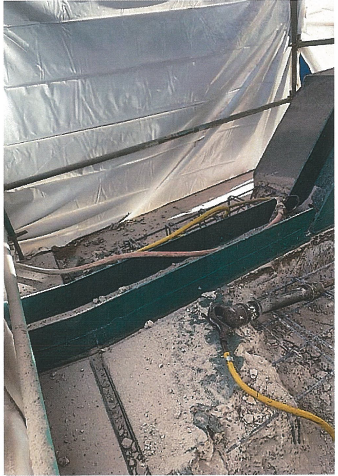
Concrete removal for diagonal support @ Section D
