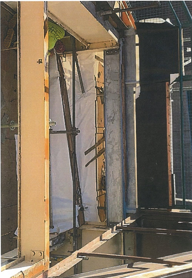
Seat Plate Replacement with Dust enclosure
